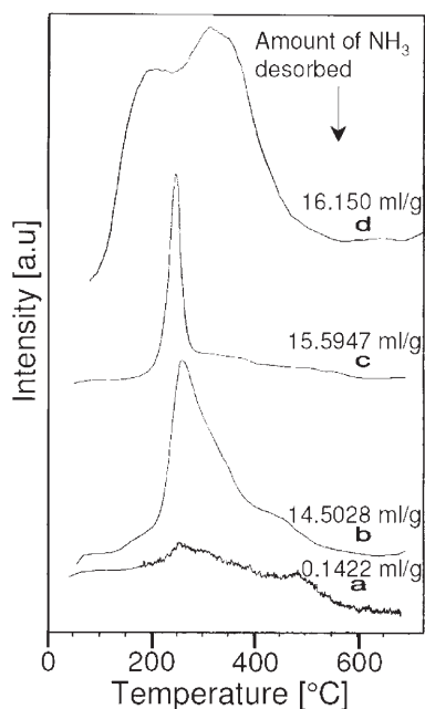
Figure 2. The ammonia TPD patterns of (a) commercial \text{TiO}_2 , (b) nano CuO, (c) nano ZnO and (d) nano \text{TiO}_2 .
