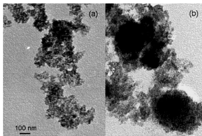
Figure 1. TEM images of the nano TiO 2 catalyst (a) before and (b) after use.
